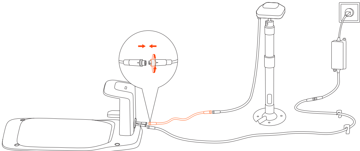
Connect the extension cable with the charging station. In case the cable is still not long enough, connect another 10 m (33 ft) extension cable. The total length of the extension cable can be 30 m (98 ft). Insert the power plug into a suitable power outlet.
